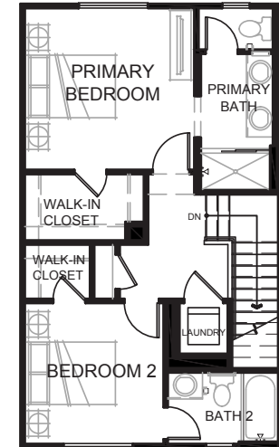
3RD FLOOR
